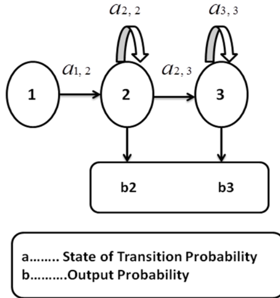
Figure 5 Three states (transition) left to right
