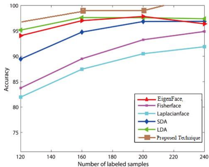
Figure 10 Comparison Results of Different Face recognition algorithms and proposed technique.
