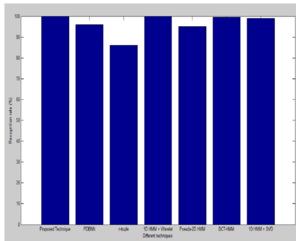
Figure 9 Comparison Results of Different Face recognition algorithms and proposed technique.
