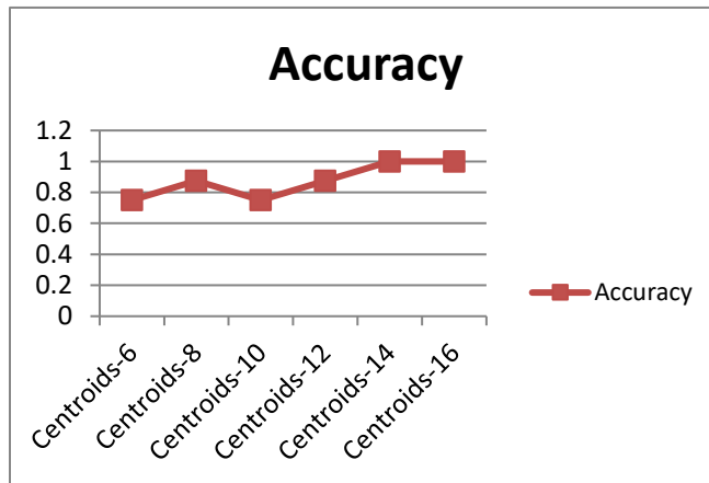
Figure.8 Accuracy versus the number of centroids.
