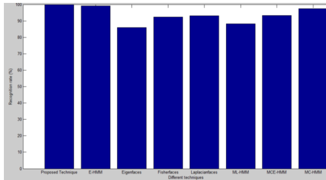
Figure 10 Comparison Results of Different Face recognition algorithms and proposed technique.
