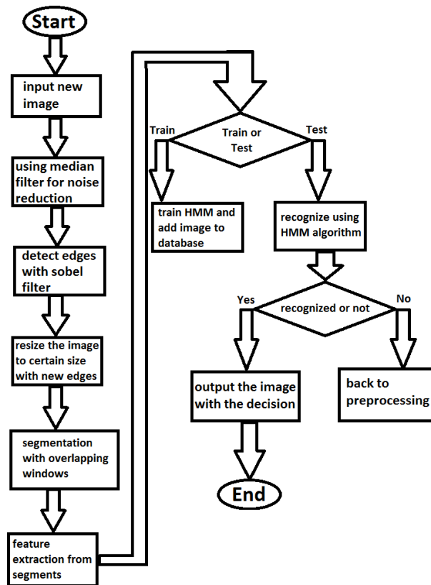
Figure 1 Face Recognition Proposed Technique
